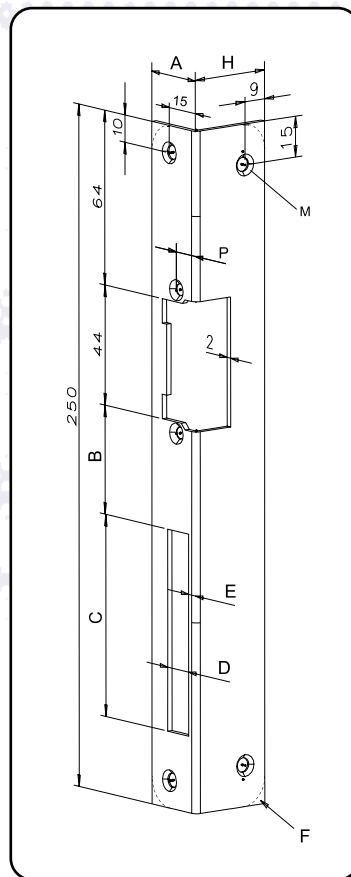
Angled striking plate 324
